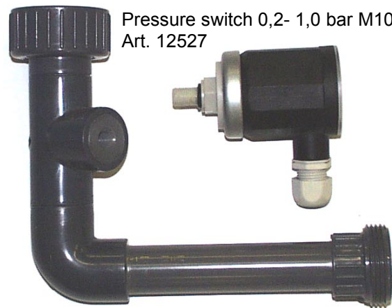
fitting filter - pump with pressure switch fitting M10x1 GR 45/100-6 Art. 12307
