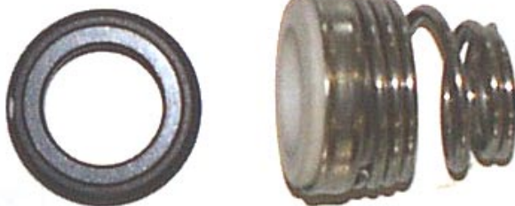
slide ring seal NTM 61 complete Art. 10333
